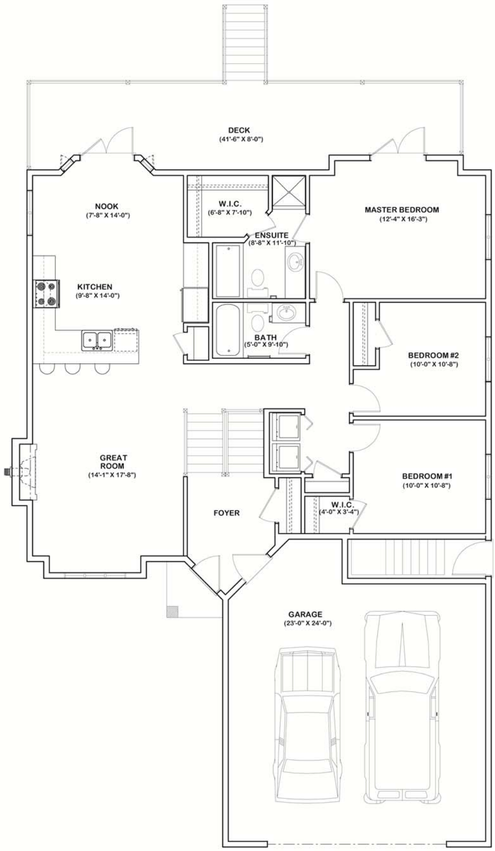
Driftwood-B MAIN FLOOR PLAN
